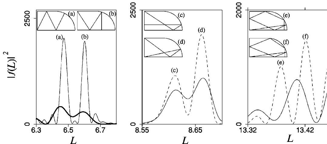
FIG. 3. |f(L)|^2 computed from the eigenvalues density of the desymmetrized stadium with Newman boundary conditions for N = 1000 (thick solid line), 2000 (thin solid line), and 8000 (dashed line), and the corresponding periodic orbits.
