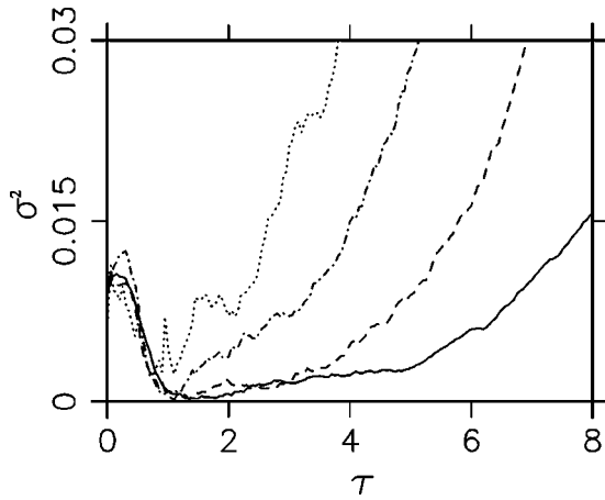
FIG. 2. Variance from the Porter-Thomas results of the wave function intensity distribution for the scar spectrum of Fig. 1, calculated using the first 1000 (dotted), 2000 (dotted-dashed), 4000 (dashed), and 8000 (full line) states of the scar spectrum of Fig. 1.
