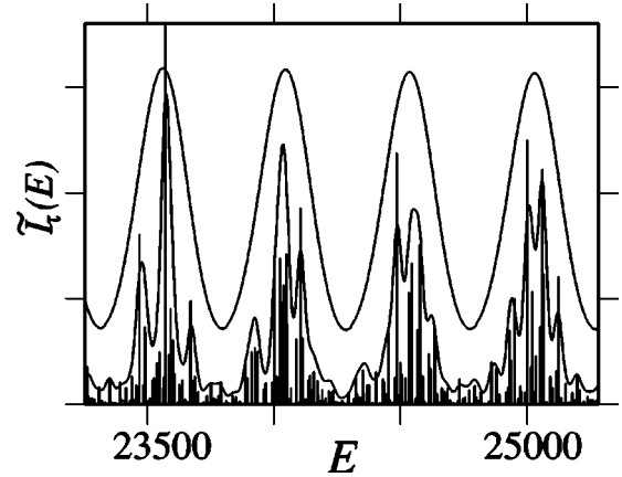
FIG. 1. Scar spectrum \tilde{I}_\tau(E) at infinite (stick) and low resolution: \tau=1 and 4.5 (solid lines), corresponding to a wave packet initially centered on the horizontal axis of a desymmetrized stadium billiard with r=1 , area 1 + \pi/4 , and Newman boundary conditions at the symmetry axes.
