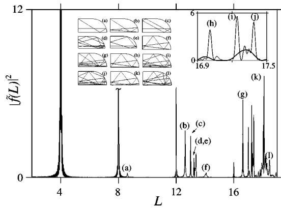
FIG. 4. |\tilde{f}(L)|^2 computed from the stick scar spectrum of Fig. 1. The different peaks have been assigned to the periodic orbits plotted in the left inset. The right inset shows how 1000 states (thick solid line) are not enough to reproduce the three central peaks of the fourth recurrence in |\tilde{f}(L)|^2 .
